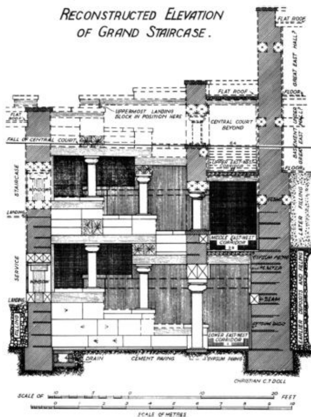
Fig. 3. Reconstructed elevation of Grand Staircase. (By Christian C.T. Doll [Evans 1921, fig. 247])
